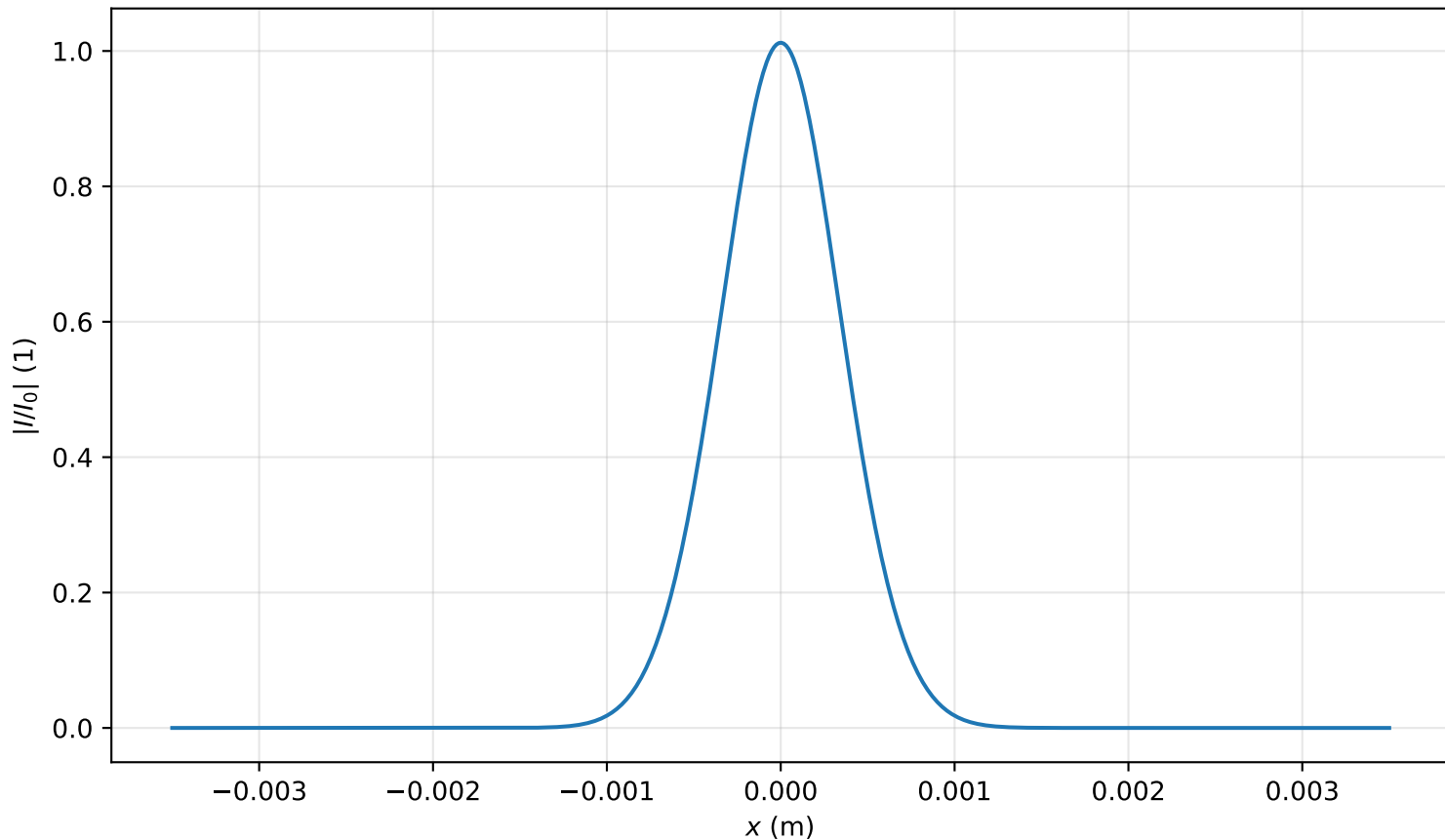
Intensity profile I(x, y = 0, z = 0.318m)/I_0 , P_{in}=0.4P_{cr} , artificial time
